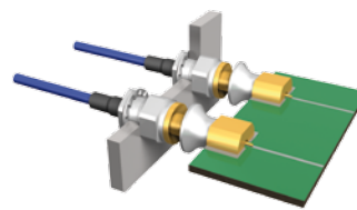
Board-to-panel connection right angle
