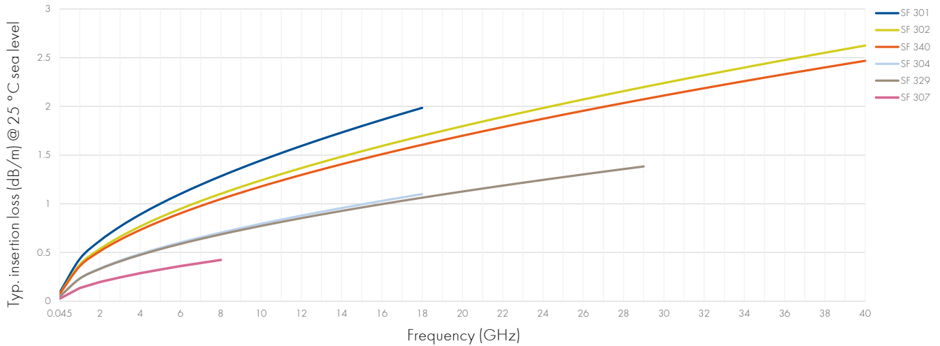
Attenuation (typical values at +25 °C ambient temperature)
