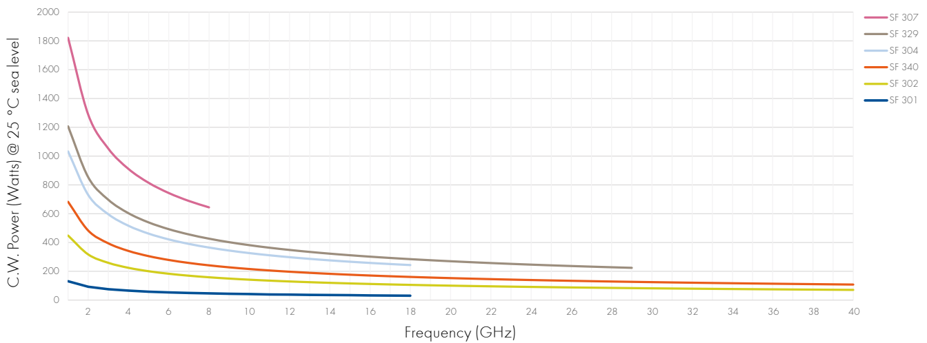
Power handling (maximum values at 25 °C ambient temperature and sea level)
