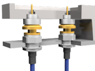
Panel-to-panel connection
