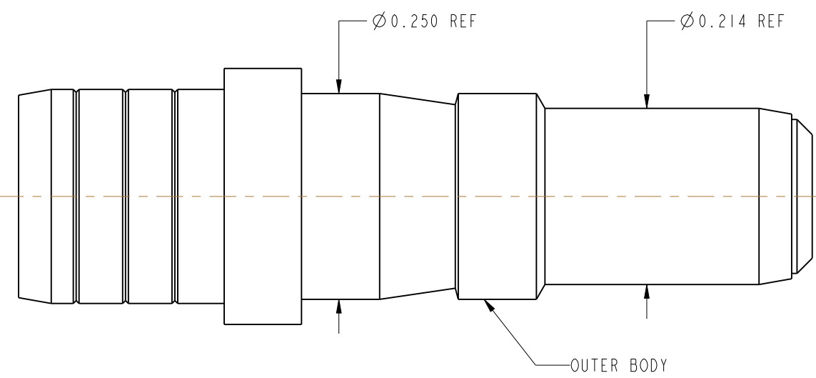
AFTER ASSEMBLY DIMENSIONS SCALE 3.000
